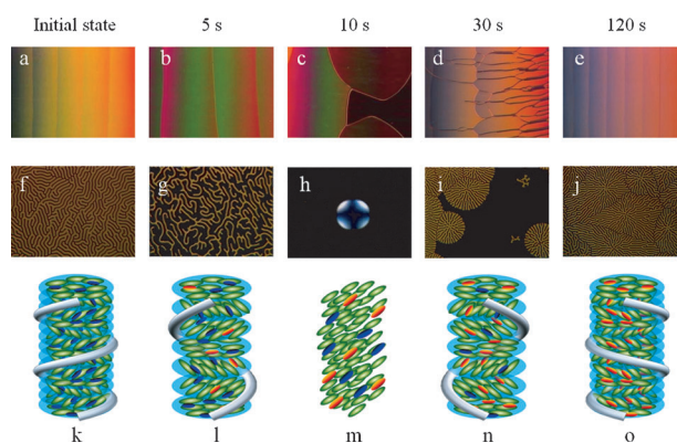
Figure 5. A change in handedness of ( S,S )- 6c (0.8 mol %) in 5CB was observed upon UV irradiation in a wedge cell (a–e) and in a homeotropic cell (f–j; conoscopic observation for (h)); illustrations of the corresponding liquid crystal phases (k–o).
